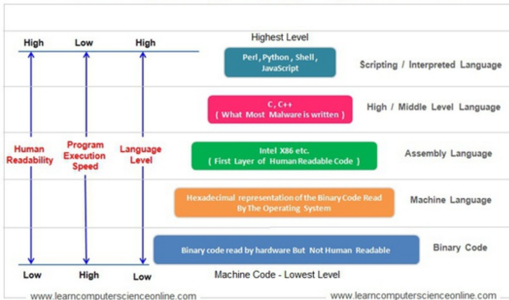
Figure 1.2: Programming languages types and levels (source: www.learncomputerscienceonline.com)
